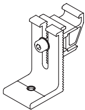
PART NAME: NOVA L-FEET PART NO.: NOVA-TRB-F16-RFN
